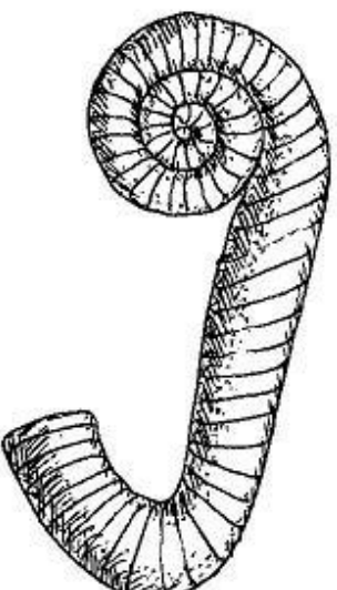
Macroscaphites (Cretaceous)
