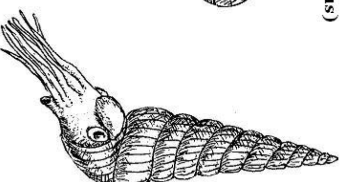
Bostychoceras (Cretaceous)
