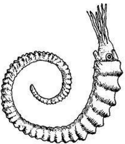
Macroscaphites (Cretaceous)
