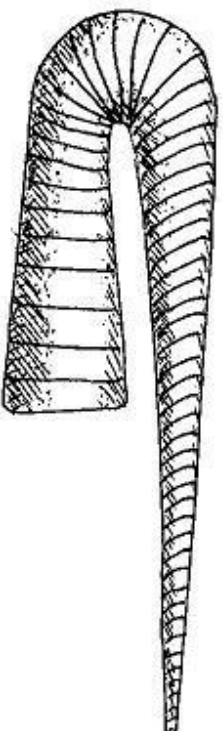
Macroscaphites (Cretaceous)
