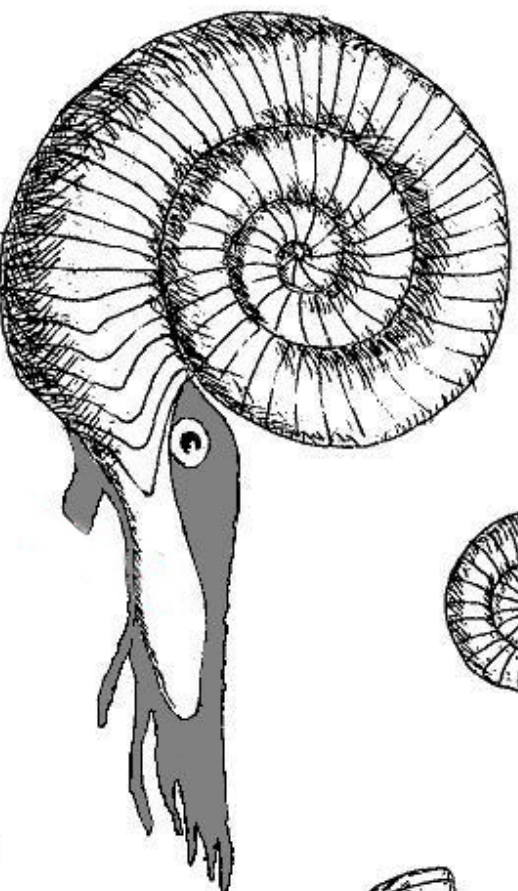
Kosmoceras (Jurassic)
